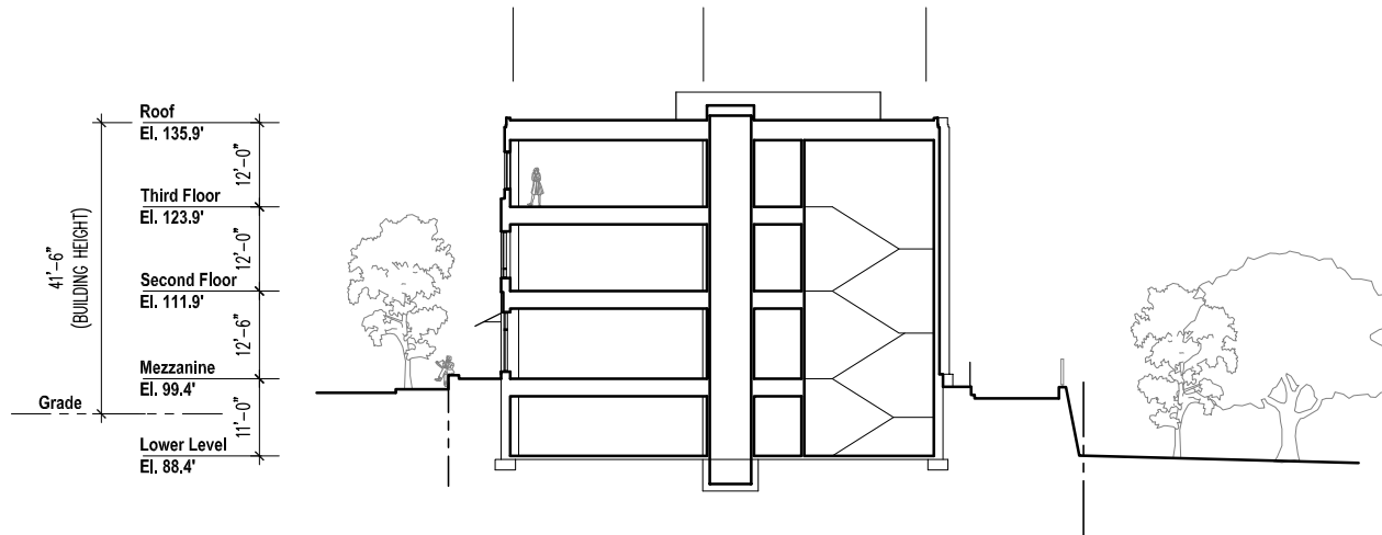
2 Parcel W - Building Section SCALE: 1" = 30'-0"
