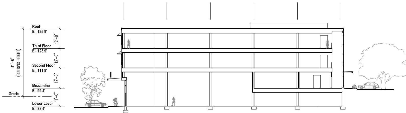
1 Parcel W - Building Section SCALE: 1" = 30'-0"
