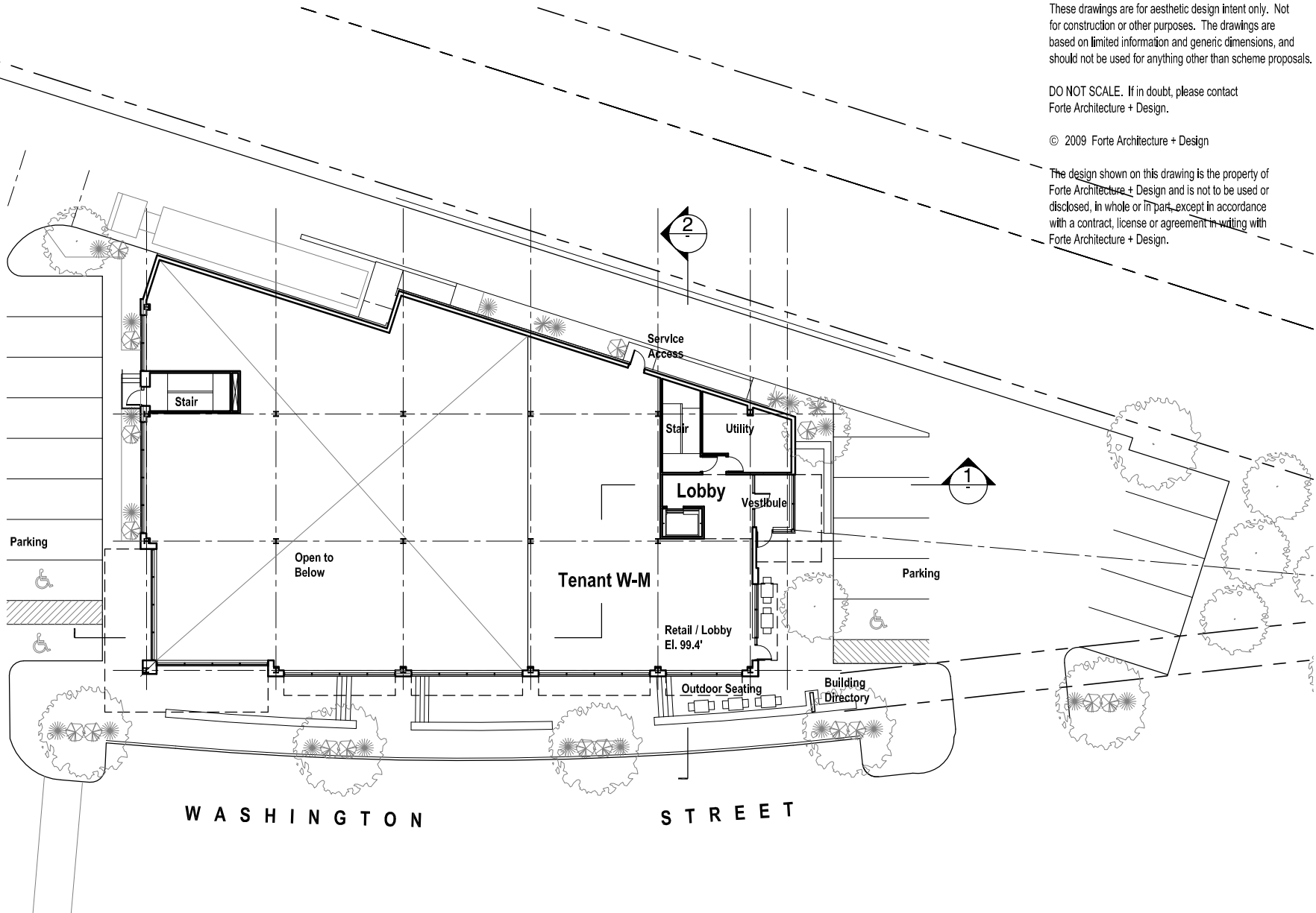
1 Parcel W - Mezzanine Level Plan SCALE: 1" = 30'-0"
