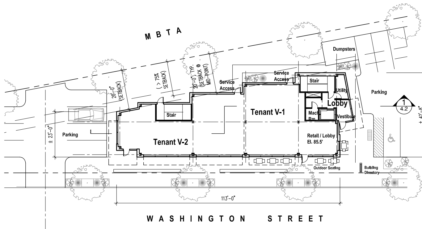
1 Parcel V - First Floor Plan SCALE: 1" = 30'-0"
